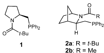
Figure 2. Pyrrolidine and azanorbornyl derivatives used as chiral ligands in asymmetric 1,4-addition.
