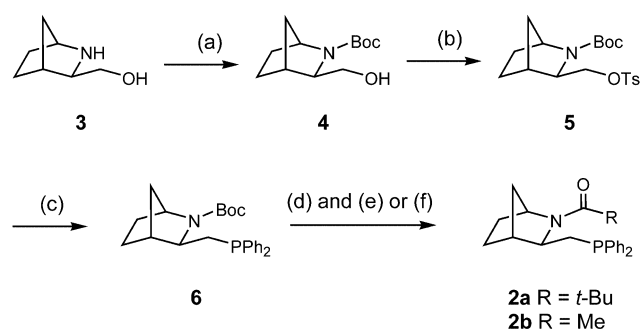
Scheme 1. (a) Et 3 N, Boc 2 O THF, rt, 88%; (b) TsCl, pyridine, CH 2 Cl 2 , 0 °C to rt, 97%; (c) LiPPh 2 , THF 0 °C to rt, 77%; (d) HCl, THF, reflux; (e) Et 3 N, t -BuCOCl, CH 2 Cl 2 , 0 °C to rt, > 98% (two steps); (f) Et 3 N, AcCl, CH 2 Cl 2 , 0 °C to rt, 83% (two steps).
